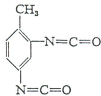
2,4-tolylene diisocyanate
