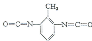
p-tolyl-1,6-diisocyanate
